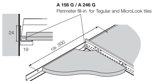
Standard perimeter finish with perimeter angle T 1924 HD or T 1924 CA
