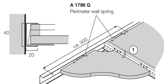
Perimeter finish with C channel T 2040 HA ① A 7890 G Universal retaining clip
