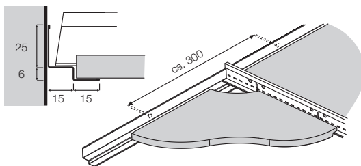
Perimeter finish with shadowline T 1506 H
