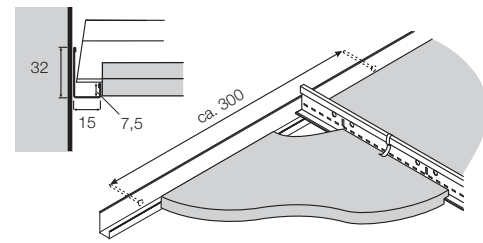
Perimeter finish with unequal U-Profile T 1575 HA
